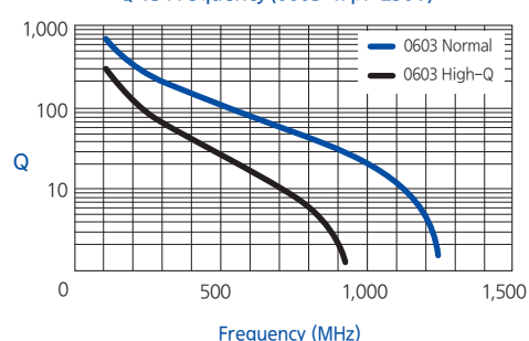
Q vs Frequency(0603 47pF 250V)
