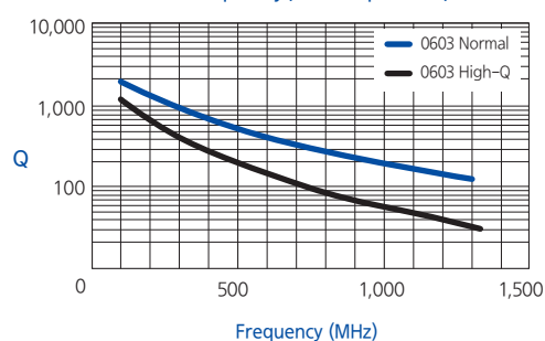
Q vs Frequency(0603 10pF 250V)
