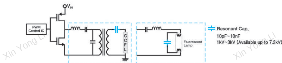
Fig. 3. Typical electronic ballast circuit and MLCC application
