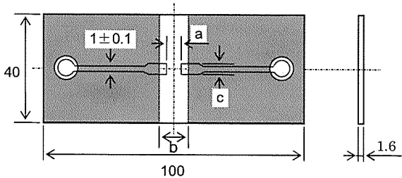
Fig.3 Test Board
