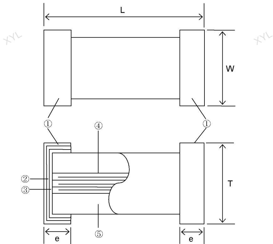
Fig.1 Shape and Dimensions
